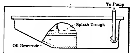
Fig. 4—Illustrating the oil pan casting of the Bergdoll with the lead to the oil pump
